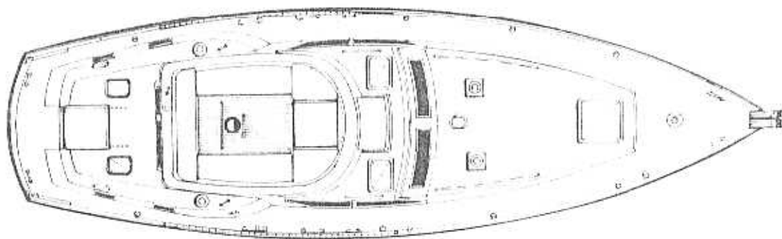
DECK LAYOUT
